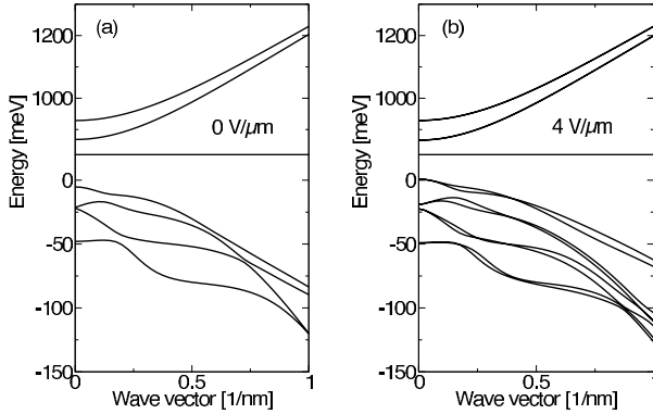
Fig. 8.1. Band structure ([100] direction) in a 13 nm InGaAsP quantum well lattice-matched to InP barriers for two different external electric fields. (a) F=0 V/ \mu m, and (b) F=4 V/ \mu m. At F=0 V/ \mu m, the valence bands are double degenerate. At F=4 V/ \mu m, they split due to the applied external electric field (Rashba effect).
