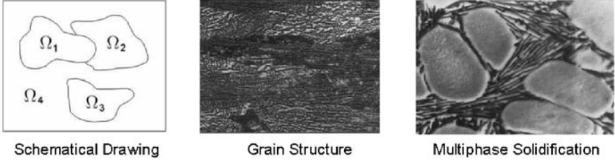
Fig. 2.1. Left image: Schematic drawing of a domain separation by four different phase regions; Middle image: Polycrystalline grain structure in Al-Si; Right image: Multiphase solidification microstructure with dendrites and a eutectic structure. (See page 683 for a colored version of the figure.)
