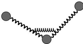
Fig. 2.2. Triatomic molecule
