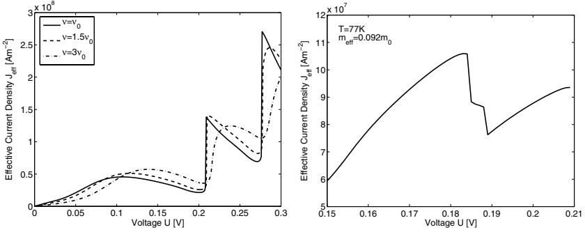
Fig. 4.4. Current voltage characteristics for a tunneling diode for the viscous QHD model. Left: isothermal case for various values of the viscosity; right: non-isothermal model.
